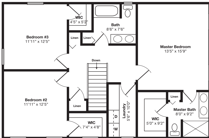
Second Floor (3 Bedroom)
